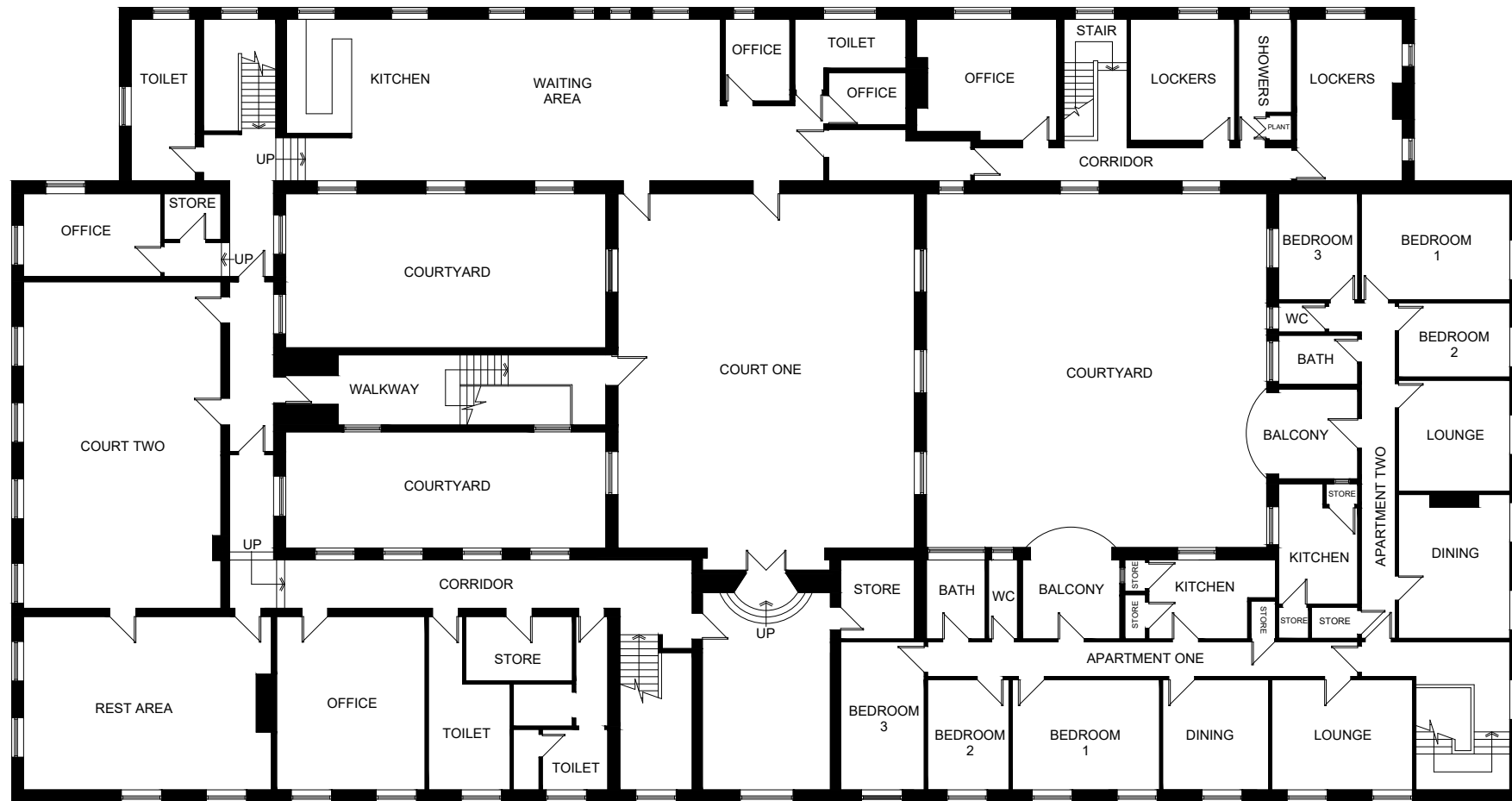
FIRST FLOOR PLAN - BLOCK A (849m 2 )
