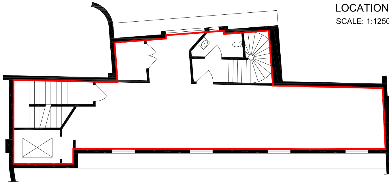
Fourth Floor
