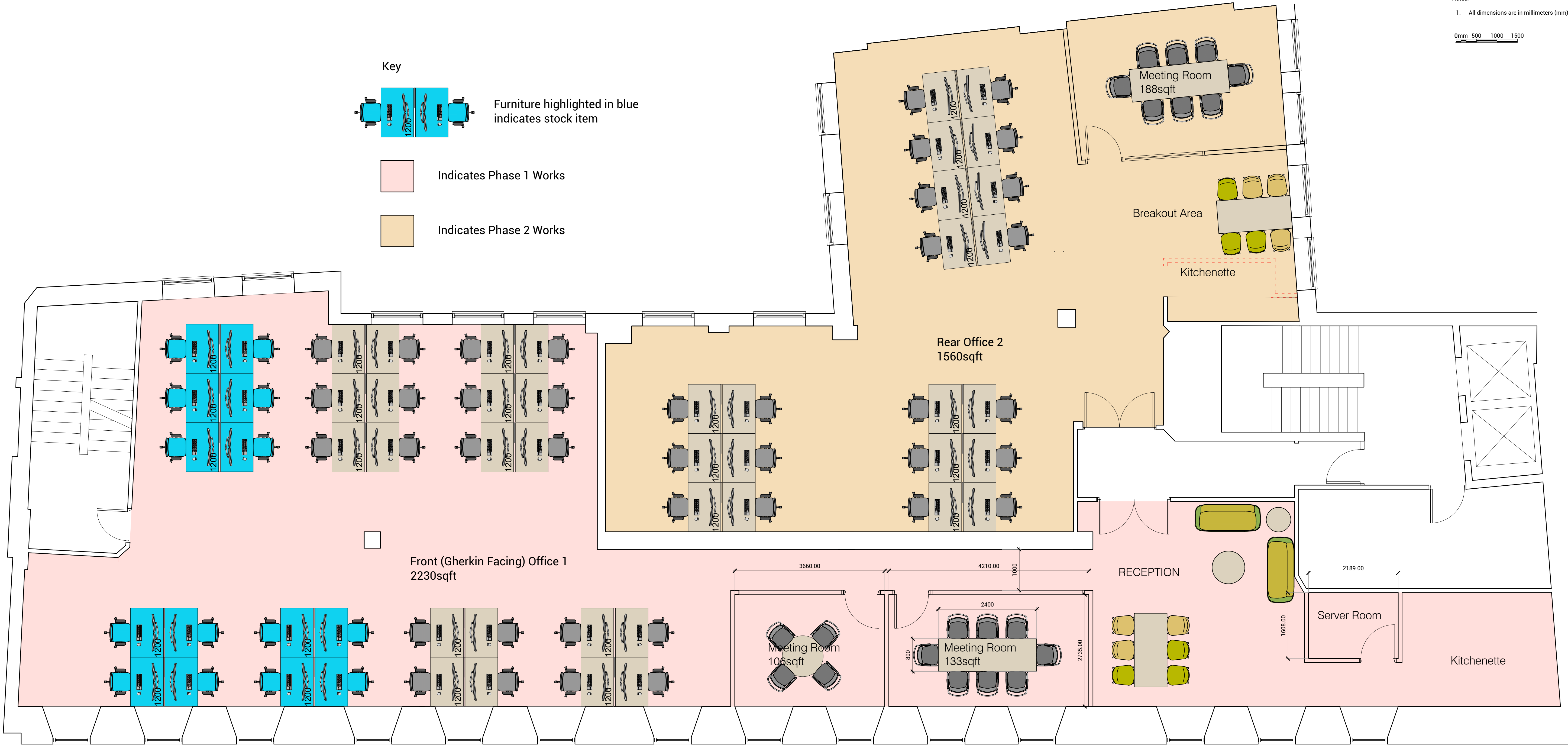
Proposed Third Floor General Arrangement Overall Plan - Sketch Scheme Option 2 Scale 1:50
